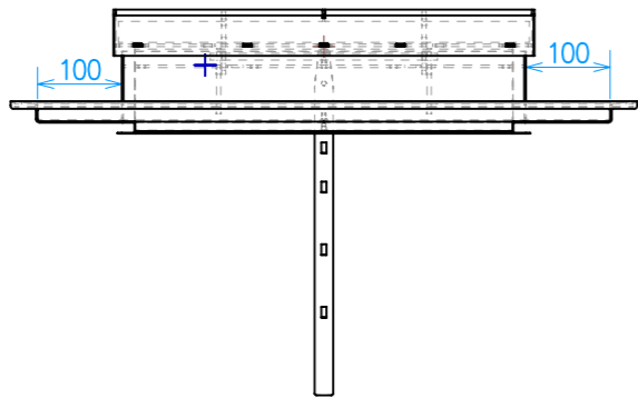
G (1:10)
