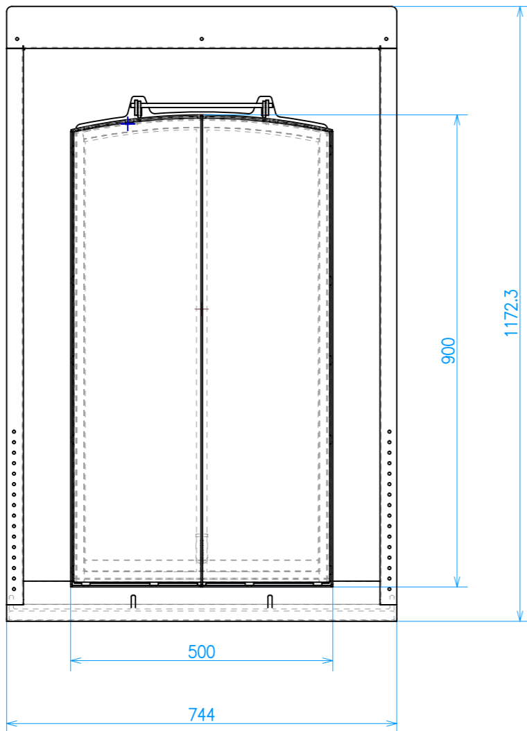
F (1:10)
